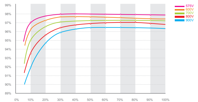
Growatt 9000UE efficiency
