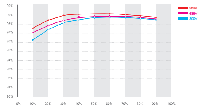
Growatt 20000TL3-HE efficiency
