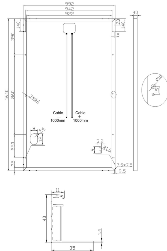
Frame Section
